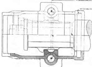
Figs. 4820-4822 Standard Journal Box and Contained Parts for Journal, 4 1/4 in. x 8 in. Plate 6.
